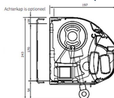
Wandmontage
